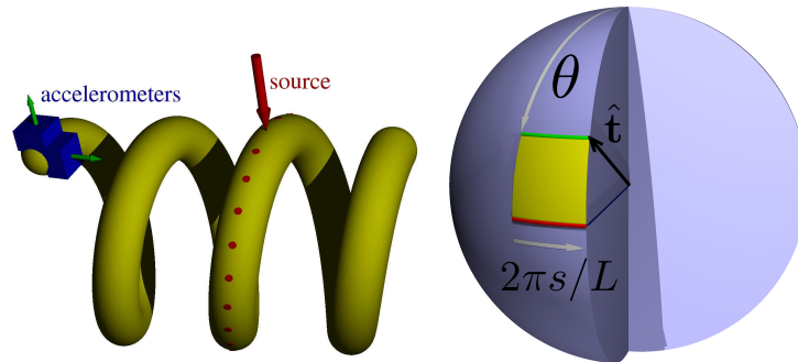
Figure 3: (Left) Setup of the experiment. Accelerometers are represented as cubes, they record acceleration in two orthogonal directions (small arrows). The large arrow symbolizes the source, a radial impact on the helix. The dots indicate some of the source positions. (Right) Geometry of the transformation from the reference trajectory to the helix trajectory. During the transformation the tangent vector for s fixed follows a meridian (vertical arrow on the figure) between colatitudes \pi/2 and \theta . A displacement of s corresponds to an azimuth angle of 2\pi s/L (horizontal arrow). The area spanned by the tangent vector during the deformation is equal to the geometric phase difference computed by Fuller's formula.
