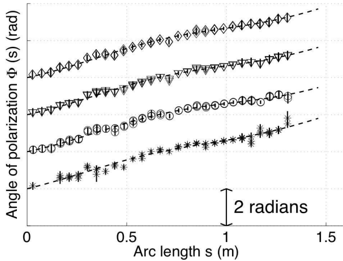
Figure 5: Measured geometric phase as a function of arc length along the helix for signals filtered at 1.4 kHz, 2.5 kHz, 4.0 kHz and 5.8 kHz. The dashed line represents the linear regression with correction for the coupling and orthogonality of the accelerometers. The origins of the curves are arbitrary.
