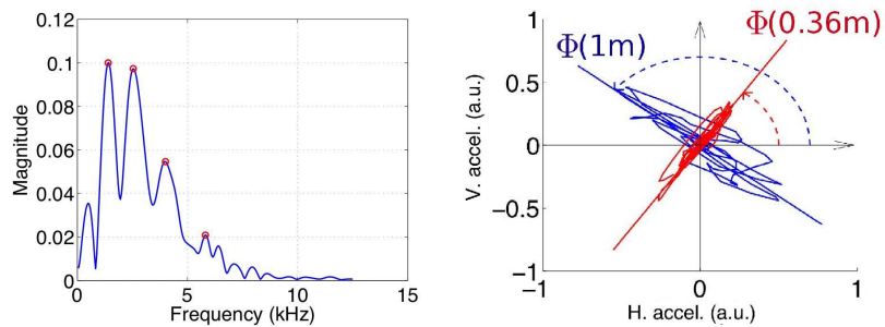
Figure 4: (Left) Power spectrum of the first oscillations of the signal corresponding to direct arrival of the flexural mode. Circles indicate the maxima used as central filtering frequencies in the signal analysis. (Right) Parametric plot of the first oscillations (direct arrival) for sources located at s = 0.36 m and s = 1.00 m. The relative angle between polarization orientations is the geometric phase difference.
