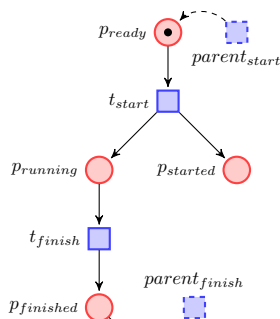
Figure 7: Petri net template for a WorkDefinition
