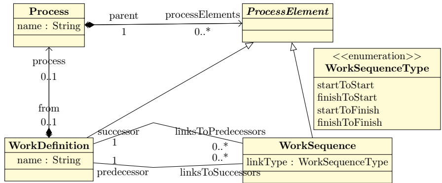
Figure 1: SimplePDL metamodel
