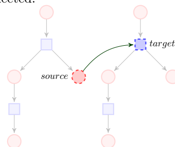
Figure 8: Petri net template a WorkSequence
