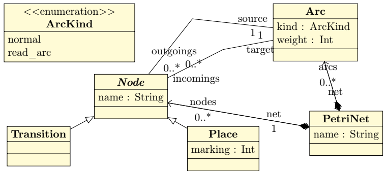
Figure 2: PetriNet metamodel
