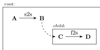
Figure 3: SimplePDL model
