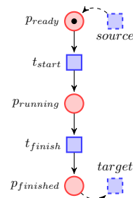
Figure 5: Petri net template for a Process
