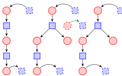
Figure 10: "Unresolved" Petri net
