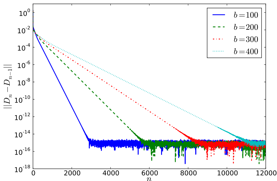
FIGURE 7.1. Convergence of the Level-Shifting algorithm. The convergence is linear until machine precision. The horizontal spacing of the curves reveals the asymptotic relationship \nu \propto \frac{1}{b} . The system considered is the carbon atom ( N = Z = 6 ), under the RHF formalism, using the 3-21G gaussian basis functions.
