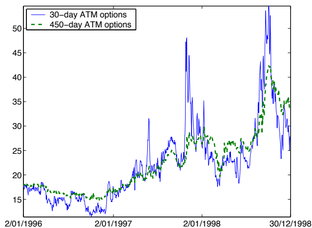
Figure 13: Implied volatility of at the money European options on CAC40 index.
