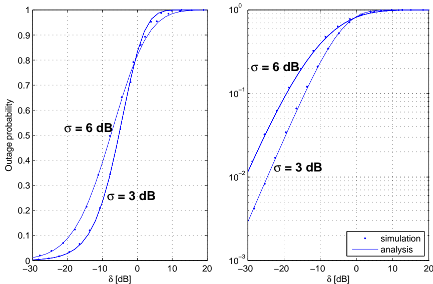
Figure 3: Outage probability for a mobile located at cell edge ( r = R_c ); comparison between analysis (solid curves) and simulations (dotted curves) on a hexagonal network ( \eta = 3 ); zoom on the right.
