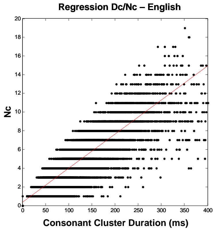
Figure 3 – Evaluation of D_c as a predictor of N_c for English. Dots are measured values and the solid line is the best linear fit estimated in the least-squares sense.
