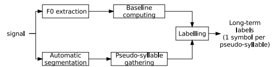
Fig. 5. Long-term coding.
