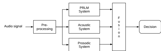
Fig. 1. Overview of the language identification system.
