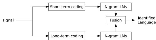
Fig. 4. Prosodic system overview.
