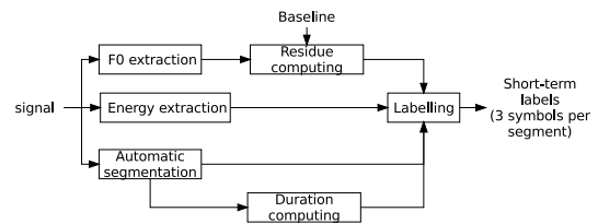
Fig. 6. Short-term coding.
