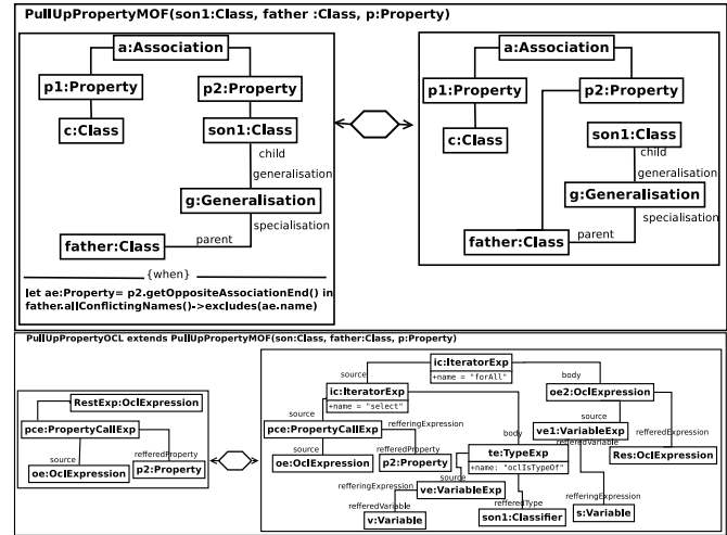
Fig. 3. QVT Rules for PullUpProperty Operation
