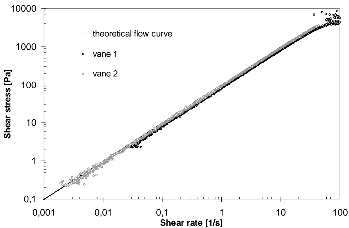
Figure 1. Vane shear flow curves prediction of silicon oil compared to its theoretical flow curve.
