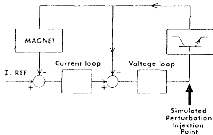
Fig 3 Block-diagram of a series-transistor converter
