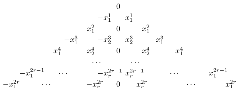
FIGURE 1. A symplectic Gelfand–Tsetlin pattern of GT_{2r}
