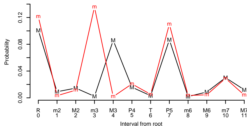
Fig. 3 Pitch probability distribution for major (M) and minor (m) chords as a function of the interval from the chord's root note.
