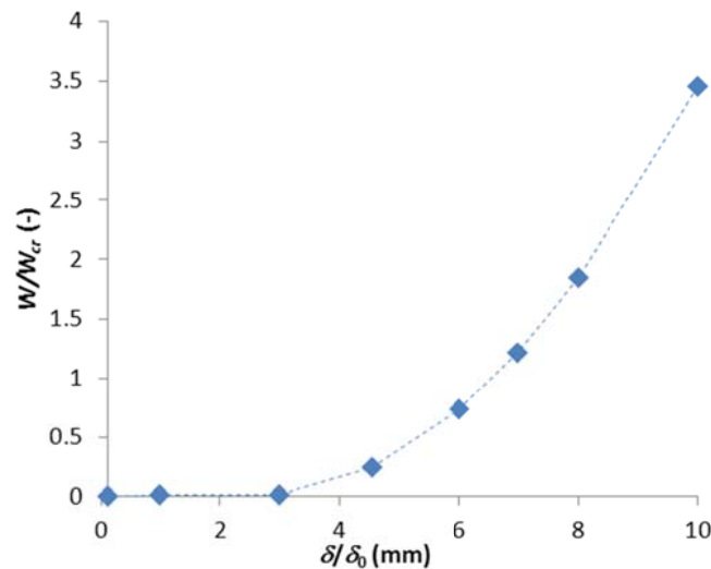
Figure 9. Evolution of W/W_{cr} at the carbonation front for \delta=d_{eff}/\kappa ratios ranging from \delta_0/10 to 10\delta_0 and for a carbonation depth of 1.35 mm.
