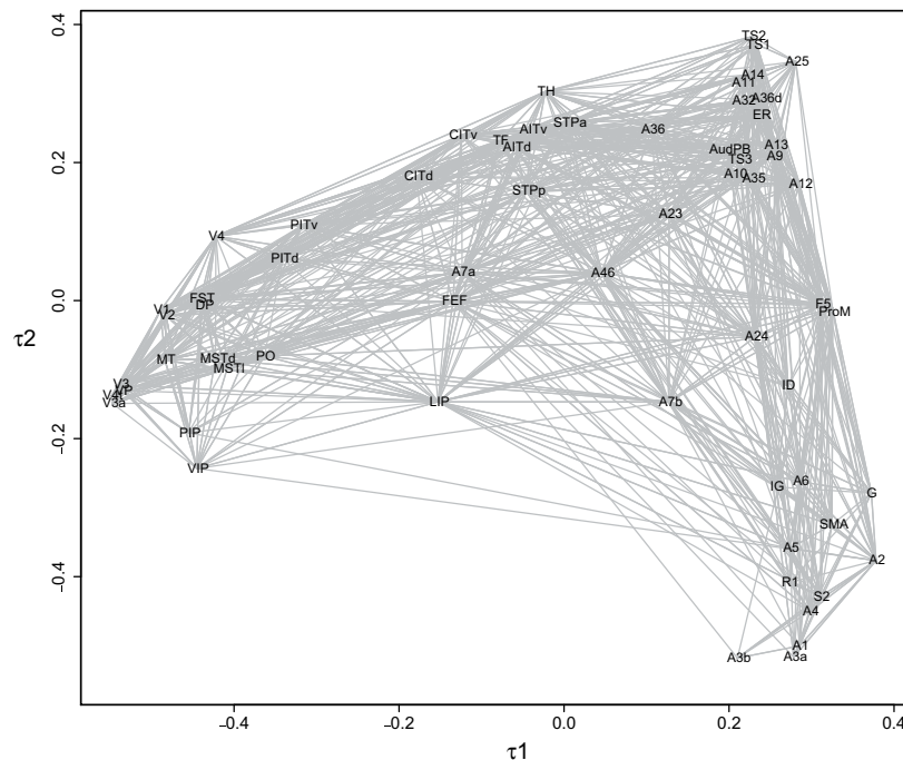
Figure 4 Topological model of cortex. Using Jouve’s algorithm (Jouve et al., 1998) on a data base of Barone (Barone et al., 2000). The network organization of the cortex can be represented as a graph, where cortical areas are nodes and the pathways between areas are the links between nodes. In this model, areas are closer according to the similarity of their connectivity.
