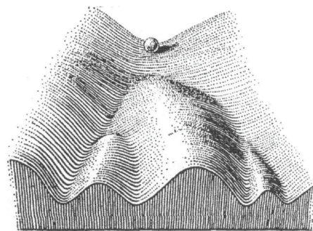
Figure 1. The Epigenetic landscape of Waddington
