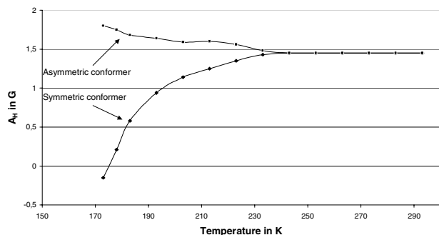
Figure 2. Variation of A_H for the two conformers of radical 1 in pentane.
