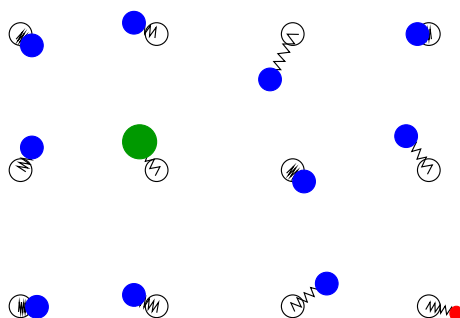
FIGURE 1. The case of nuclei on a lattice whose charges and positions are perturbed by i.i.d. random variables. A Gaussian displacement (10) corresponds to having the nuclei attached to harmonic oscillators vibrating randomly and independently, according to their Gibbs measure.
