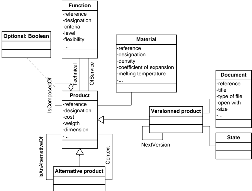
Fig. 4: UML class diagram of the product meta-model
