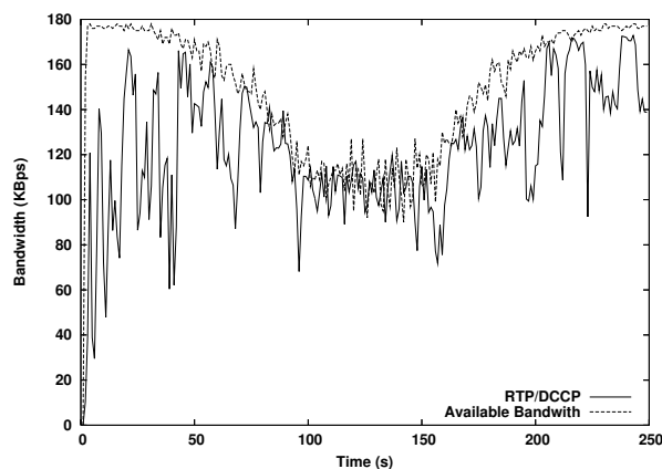
Figure 5: Throughput comparison.
