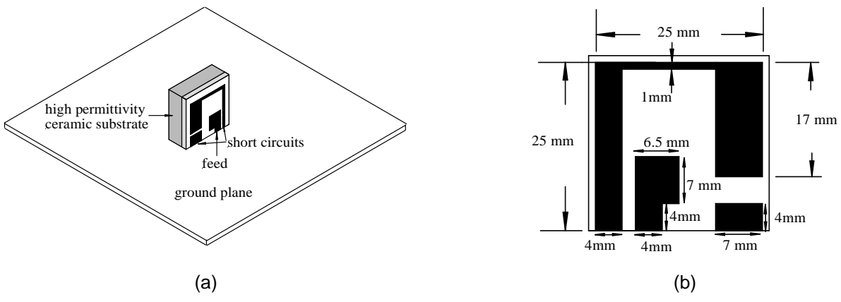
Figure 2 : Overview of the narrow band antenna represented by the association of a printed antenna and a ceramic substrate (a) and a zoom of the radiating element with its main dimensions (b).
