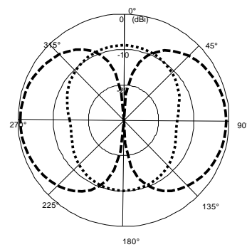
(b) DC voltage : 0V, f = 470 MHz (...) E_{\phi} and E_{\theta} (--) in XZ plane
