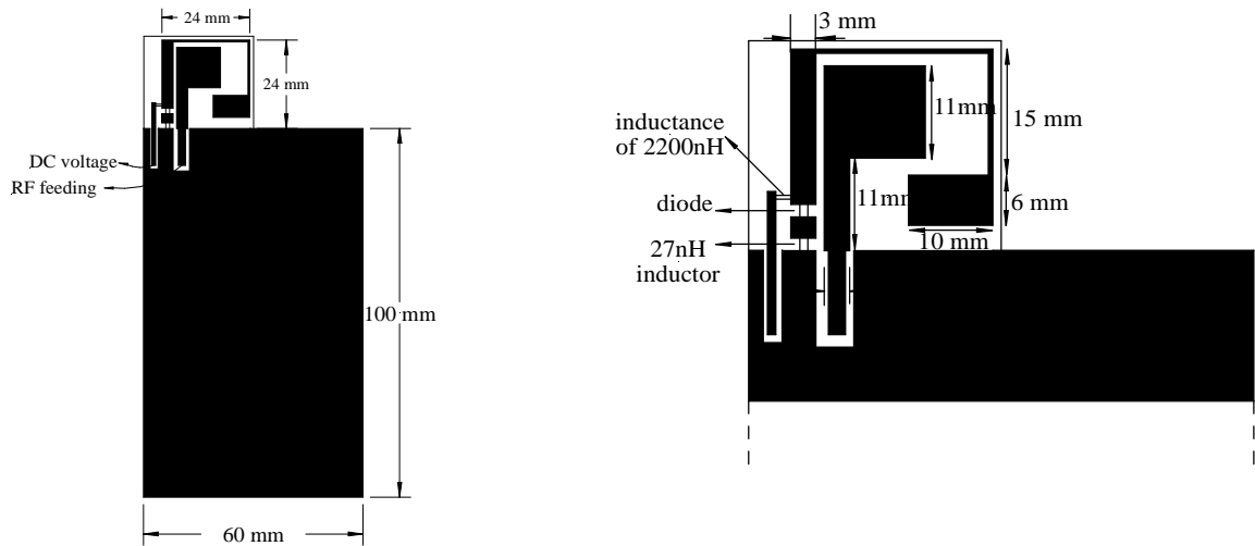
Figure 4 : Overview of the frequency tunable antenna with the circuit board simulating the mobile circuit board (a) and a zoom of the antenna with the DC bias circuit.
