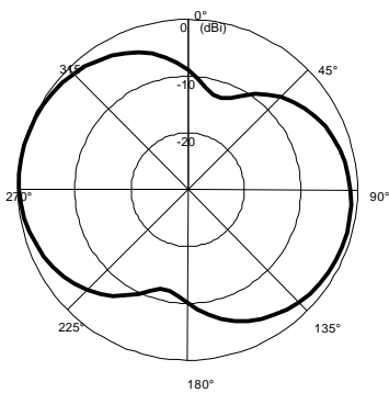
(a) DC voltage : 0V, f = 470 MHz (-) E_{\theta} in YZ plane
