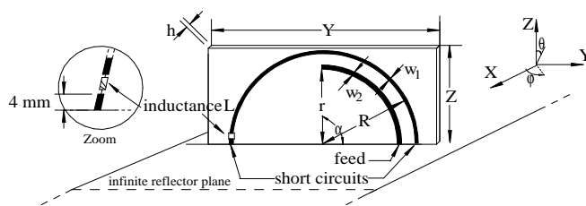
Figure 1 : Geometry of the MCLA
