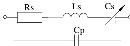
Figure 5 : Equivalent circuit models of the varactor diode
