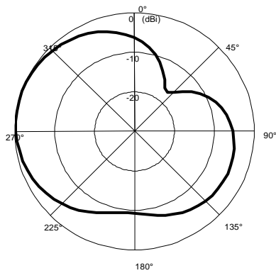
(e) DC voltage : 2V, f= 710 MHz (-)E \theta in YZ plane
