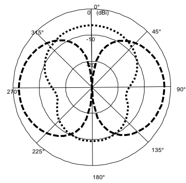
(f) DC voltage : 2V, f= 710 MHz (...)E \phi and E \theta (-) in XZ plane
