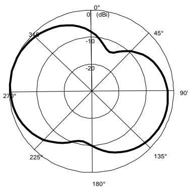
(c) DC voltage : 1.5V, f = 620 MHz (-) E_{\theta} in YZ plane
