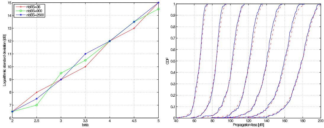
Fig. 1: Left: Critical values of \sigma_{\text{dB}(S)} , above which, the empirical distribution of L^* in the hexagonal network cannot be distinguished from this for the “equivalent” Poisson model (cf. Section II-E). Right: Visual comparison of the cdf’s for the hexagon model of 6 \times 6 = 36 BS and the Poisson one for \beta = 2, 2.5, 3, \dots, 5 (curves from left to right) for the corresponding critical values.
