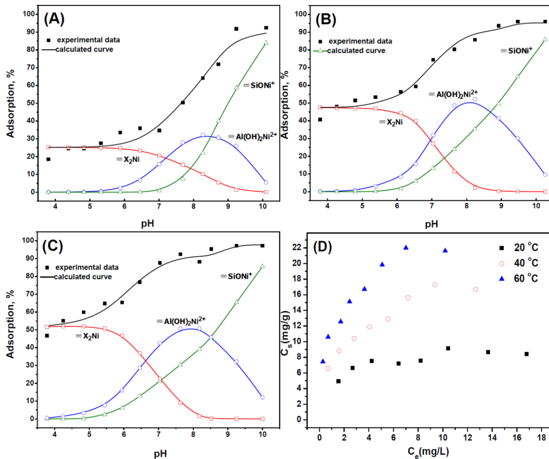
Fig. 2 Sorption percent of Ni(II) on Ca-montmorillonite and corresponding surface species repartition diagrams at temperature 20°C (A), 40°C (B), 60°C (C). Sorption isotherms of Ni(II) on Ca-montmorillonite at three temperatures (D). m/V=0.5 g/L, I=0.001 mol/L Ca(NO_3)_2 . (A-C): C_{Ni(II)initial}=10 mg/L; (D): pH=6.4.
