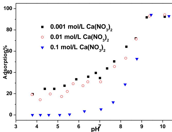
Fig. SI-2 Sorption edges of Ni(II) at different ionic strengths. m/V = 0.5 g/L, C_{\text{Ni(II)initial}} = 10 mg/L, T = 20 °C and I = 0.001, 0.01 and 0.1 mol/L \text{Ca}(\text{NO}_3)_2 .
