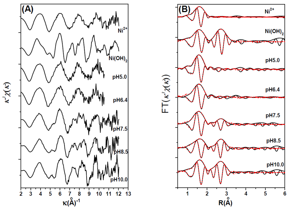
Fig. 3 Raw k^3 -weighted \chi(k) spectra of references and experimental samples (A) and their corresponding pseudo radial distribution functions (RDFs) (B) at different pH. m/V=0.5 g/L, C_{\text{Ni(II)initial}}=10 mg/L, pH=5.0, 6.4, 7.5, 8.5 and 10.0, T=20^\circ\text{C} , I=0.001 mol/L \text{Ca}(\text{NO}_3)_2 .
