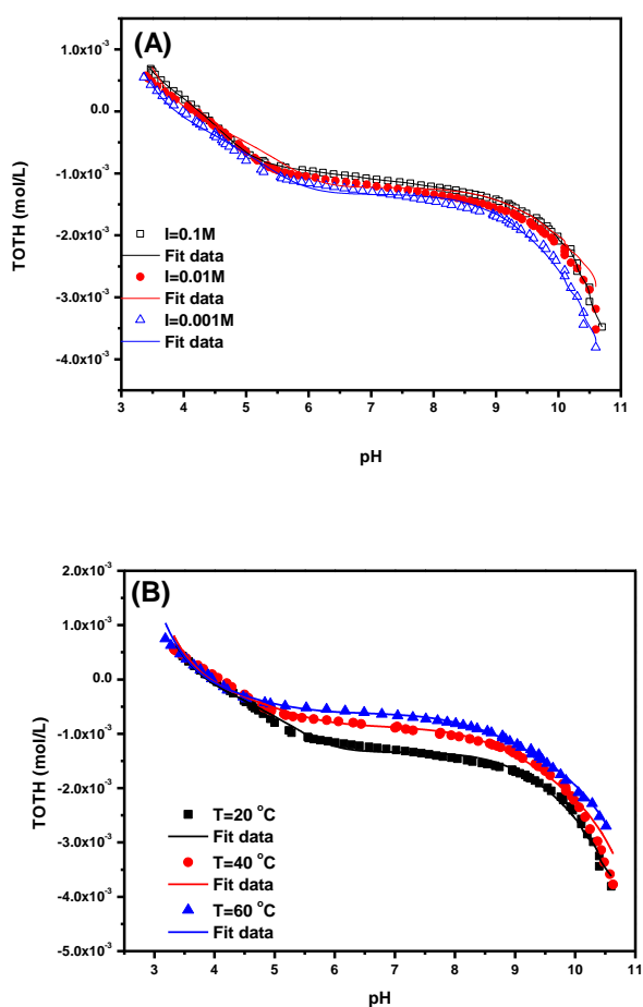
Fig. SI-1 Acid-base titrations of Ca-montmorillonite (5.0 g/L) as a function of pH in 0.001, 0.01 and 0.1 mol/L \text{Ca}(\text{NO}_3)_2 at T = 20\text{ °C} (A) and at three different temperatures in 0.001 mol/L \text{Ca}(\text{NO}_3)_2 (B). The lines are calculated using FITEQL 3.2.
