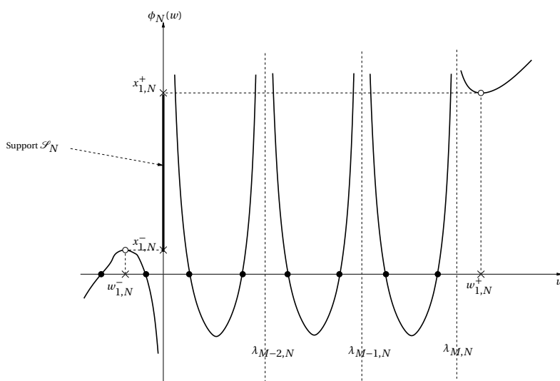
Figure 2.2: \phi_N(w) : Case 1
