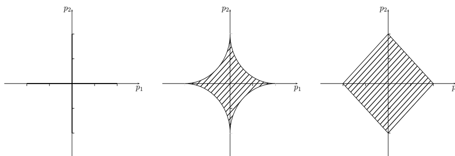
FIGURE 2. Z(x) for x = 0 , 0 \leq |x| \leq 1 and |x| \geq 1 respectively.
