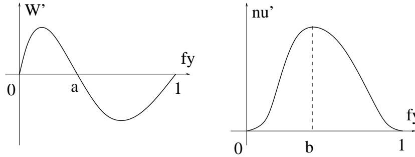
Figure 1: Derivatives of the double-well potential W and of the entropy coefficient \nu .
