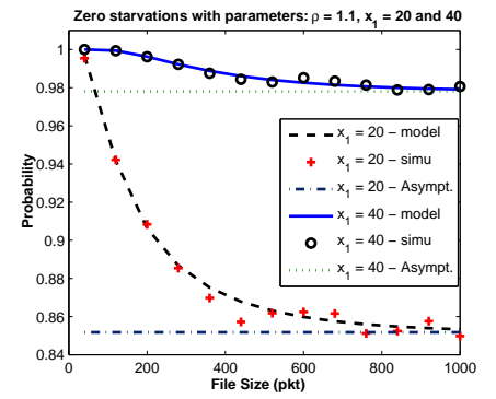
Fig. 4. Probability of no starvation with \rho = 1.1 : x_1 = 20 and x_1 = 40
