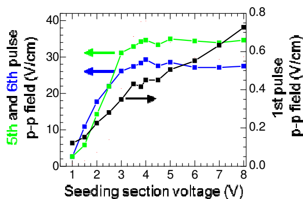
Figure 3 Maximum peak-to-peak (p-p) fields of the 1st (black), fifth (green) and sixth (blue) THz pulses versus the voltage applied to the seeding facet. For values of the seeding voltage > 4 \text{ V} , the amplitudes of the fifth and sixth THz pulses saturate, while the amplitude of the 1st THz pulse continues to increase.
