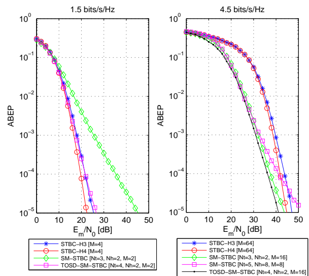
Fig. 2. ABEP against E_m/N_0 . Performance comparison with STBC-H3 and STBC-H4 [19] codes for a rate of 1.5 bits/s/Hz (left) and 4.5 bits/s/Hz (right).
