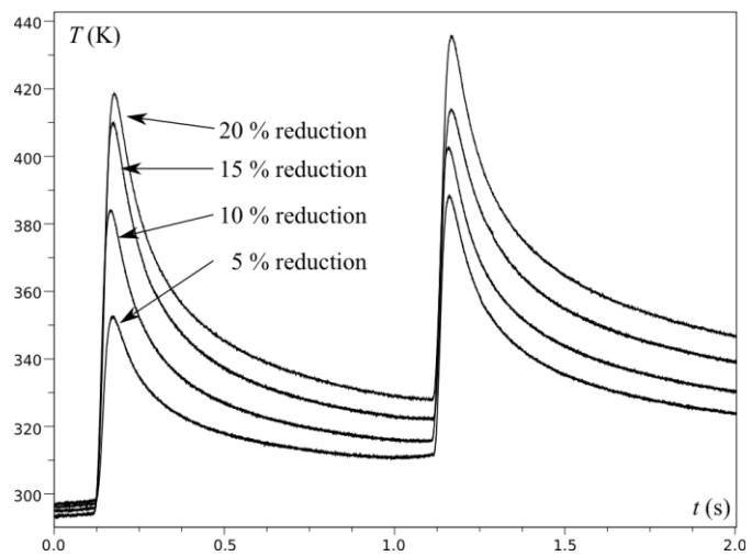
Fig 5. Temperature measurements for various reductions
