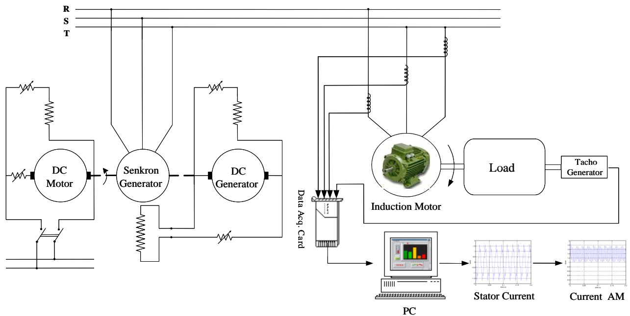
Fig. 6. Test facility.
