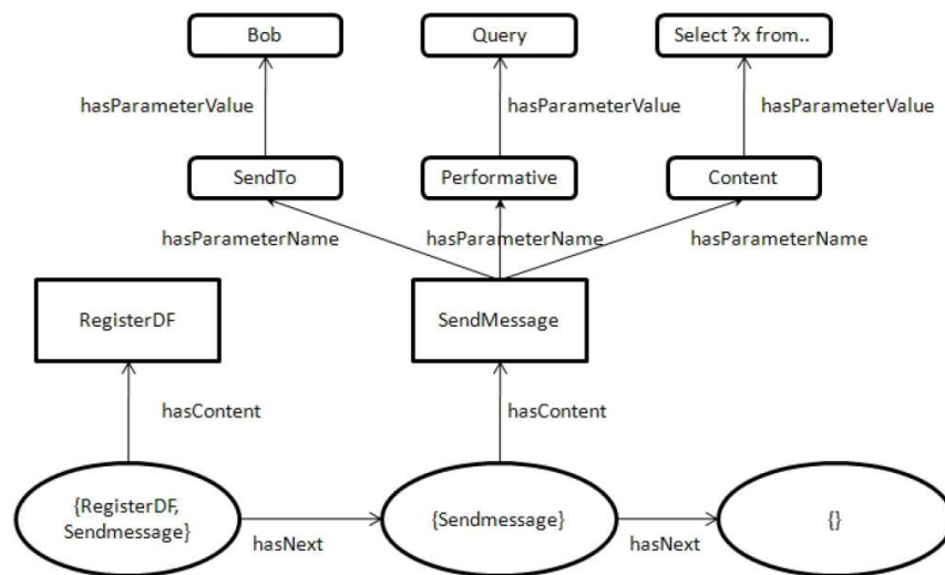
Fig. 1.11 Illustrative example (b), ActionList data structure
