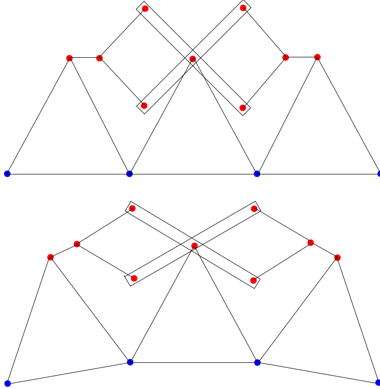
Figure 11. The basic element of the 3rd gradient beam and its major floppy mode.
