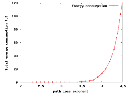
Fig. 3. Energy consumption vs path loss exponent : Idle=0.4*RX .
