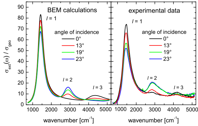
Fig. 3: Experimental extinction cross section ( \sigma_{\text{ext}} , derived from transmittance as in Ref. 10 and 12, normalized to the geometric cross section \sigma_{\text{geo}} ) of a nanorod with w \approx h \approx 60 nm, compared to BEM calculations for a cylindrical nanorod ( D = 68 nm, \pi D^2 = 4wh ) of the same length L = 1500 nm for various incident angles \alpha as indicated.
