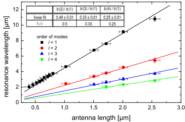
Fig. 2: Relation between \lambda_{\text{res}} and length L for different orders l . The solid lines are linear fits of \lambda_{\text{res}} = b(l)L/l to the experimental data with the fit parameter b(l) for the l^{\text{th}} order. The inset-table compares b(l)/b(l=1) to the ideal ratio 1/l . The error bars indicate the experimental error in the resonance frequency and length as estimated from SEM images.
