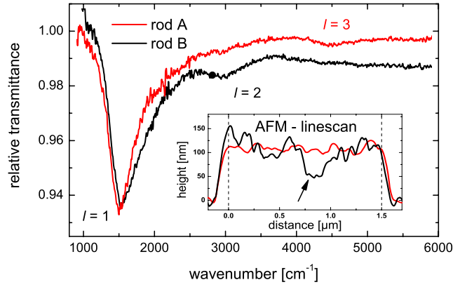
Fig. 1: Relative IR transmittance spectra of two similarly prepared nanorods (A, B) with L \approx 1500 nm, w = 60 nm and h = 100 nm. The resonance order l is indicated. The inset shows AFM height profiles along the rod's long axis. The main defect of nanorod B is indicated with an arrow.
