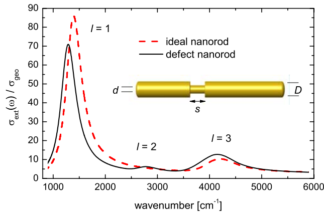
Fig. 4: Simulated extinction spectra of an ideal (red line) and an inhomogeneous (black line) nanorod with L = 1500 nm and D = 60 nm. The detailed shape of the nanorod with defects is shown in the inset ( d = 30 nm, s = 100 nm, the neck position is 155 nm away from the rod center).
