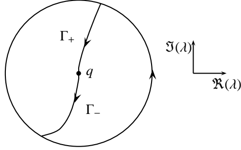
Figure 4: Contours in the RHP for \tilde{\mathcal{P}} .
