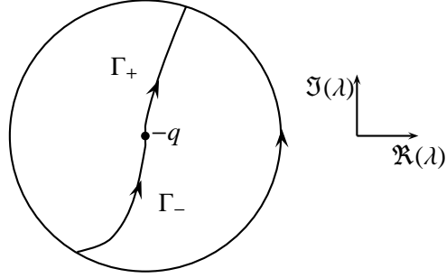
Figure 3: Contours in the RHP for \mathcal{P} .
