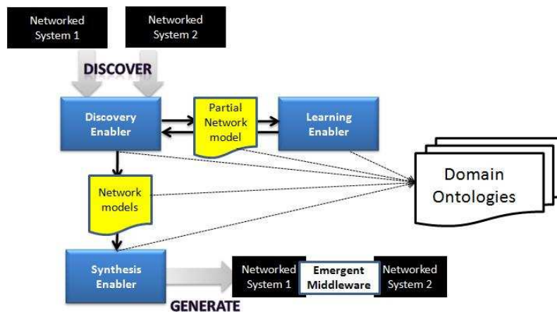
Fig. 3. The architecture of the emergent middleware Enablers
