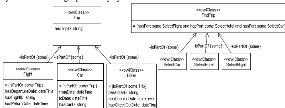
Fig. 4. The travel agency ontology
