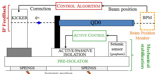
Figure 1: Overall layout of the FF stabilization.
