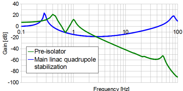
Figure 2: Transfer function of ML quadrupole stabilization and preisolator.
