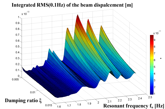
Figure 13. Integrated RMS(0.1Hz) versus mechanical support characteristics.
