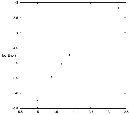
Figure 9: Error in discrete uniform norm for \phi (left) and \psi (right) with \Delta t = \frac{1}{300} and different values of \Delta x . The reference solution has been calculated with \Delta x = 2\Delta t = \frac{1}{300} .
