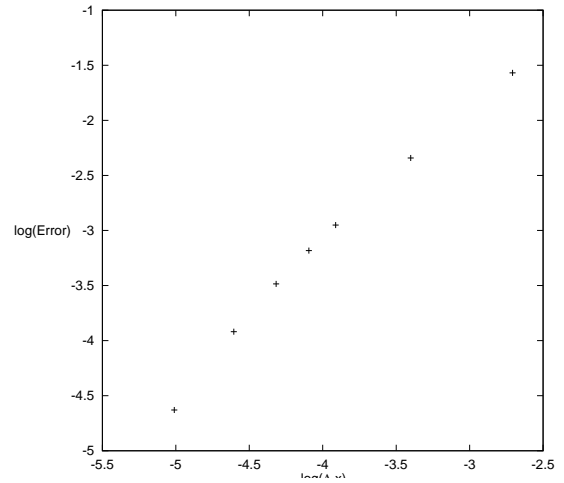
Figure 9: Error in discrete uniform norm for \phi (left) and \psi (right) with \Delta t = \frac{1}{300} and different values of \Delta x . The reference solution has been calculated with \Delta x = 2\Delta t = \frac{1}{300} .
