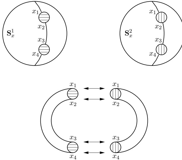
FIGURE 3. Construction of the Riemann surface
