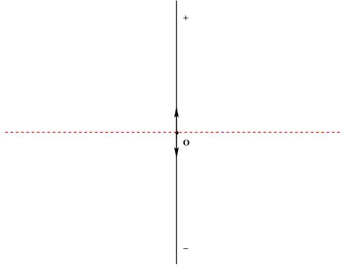
Figure 3: SBM equation.
