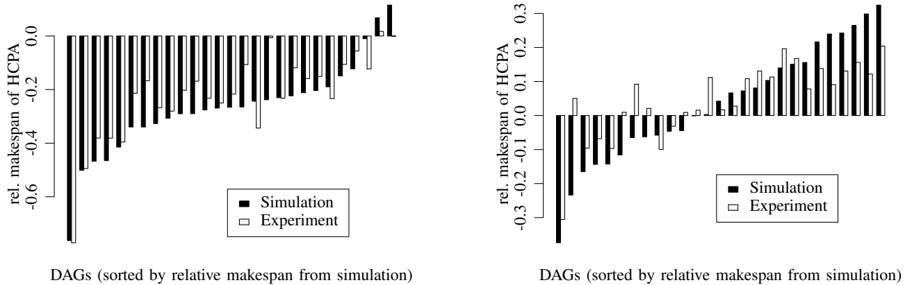
Figure 7. HCPA makespan relative to that of MCPA using empirical models. Left-hand side: n = 2,000 . Right-hand side: n = 3,000 .
