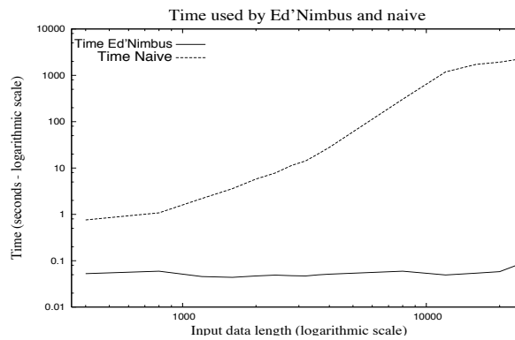
Fig. 2. Time spent by ED’NIMBUS and the naive algorithm w.r.t. the input size, in logarithmic scale. In all tests there are 4 input sequences of growing size ( x axis), and we filter (100, 4, 10) -repetitions, with k = 6 .
