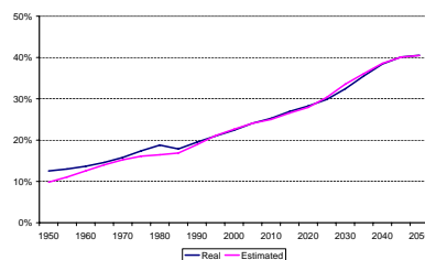
Figure 8: >65 / >20
