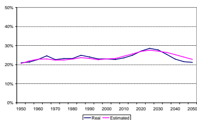
Figure 7: 50-64 / >20
