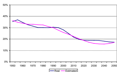
Figure 5: 20-34 / >20
