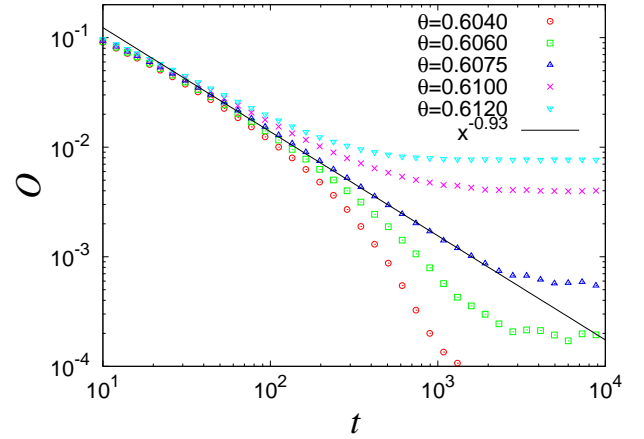
FIG. 3. (Color online) Variations of O versus time t , shown for different \theta values. At critical value \theta_c , order parameter follows a power law decays with exponent \delta \simeq 0.93 (shown by the solid line). ( N = 10^7 ; Mean field model with average taken over many independent initial conditions).
