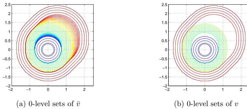
Figure 2: Case 2: Numerical solutions with 150^2 grid nodes.
