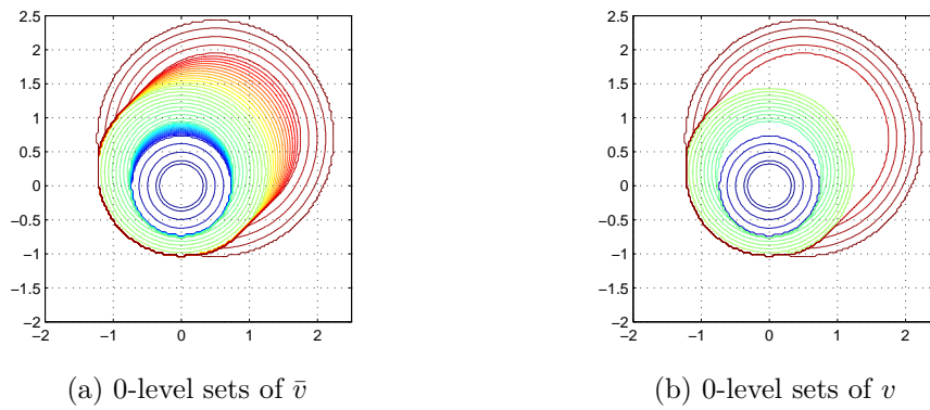
Figure 1: Case 1: Numerical solutions with 150^2 grid nodes.
