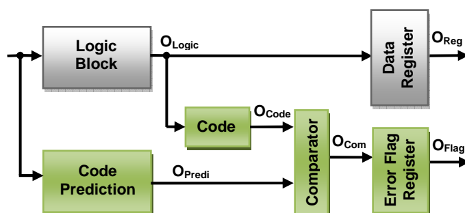
Figure 1. A state-of-the-art CED code-based scheme
