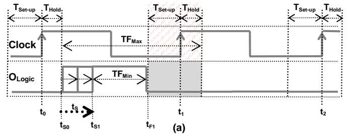
Figure 3. STF-TIs on O_{Logic} for which a Data Register's FF certainly manifest a SISE-STF-LWNV – i.e. FC1
