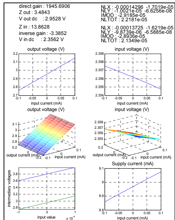
Figure 3: Macro-model DC parameters extraction
