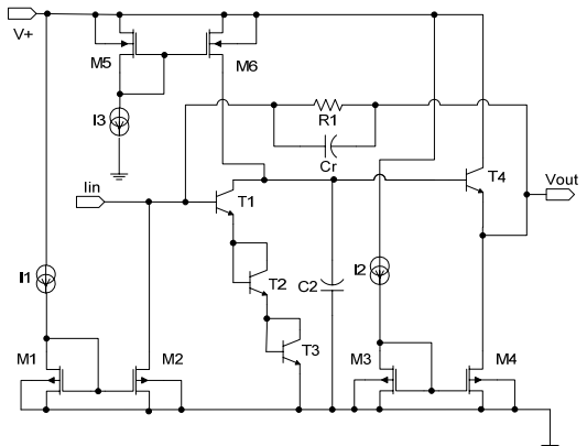
Figure 6: Transimpedance amplifier with real sources
