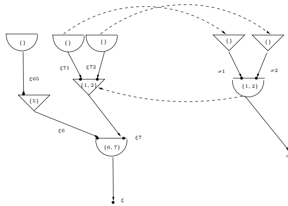
Figure 8: A J-proof structure R_1 labelled with actions
