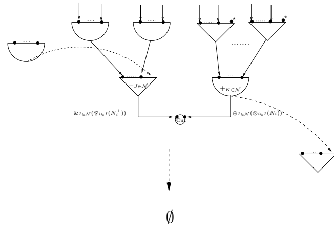
Figure 26: +_{K \in \mathcal{N}} / -_{J \in \mathcal{N}} cut reduction (with J \neq K ).
