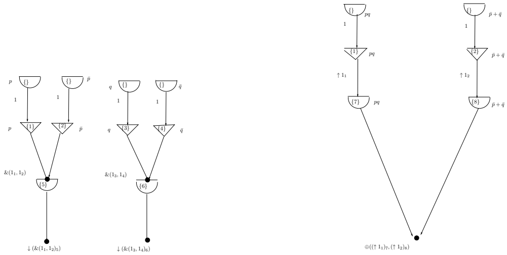
Figure 34: Non-monomial labelling
