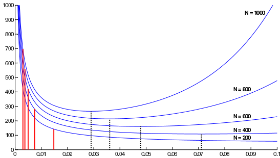
Fig. 11. Mean scattering time [in min] with respect to \alpha . N_{\text{sup}}/N = 80\% , N_{\text{inf}}/N = 20\% , K = 3 and \mu = 1 \text{ min}^{-1} . For each curve, the vertical solid line corresponds to the critical value \alpha_c , while the dotted line corresponds to \alpha_{\text{min}} (whenever it is less than the right bound of the axis).
