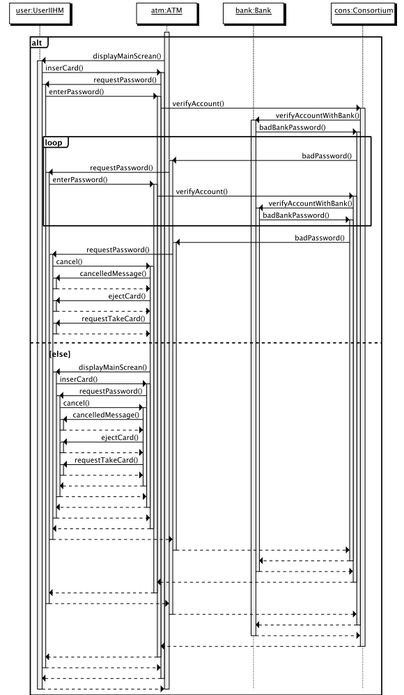
Figure 6. The extracted sequence diagram.
